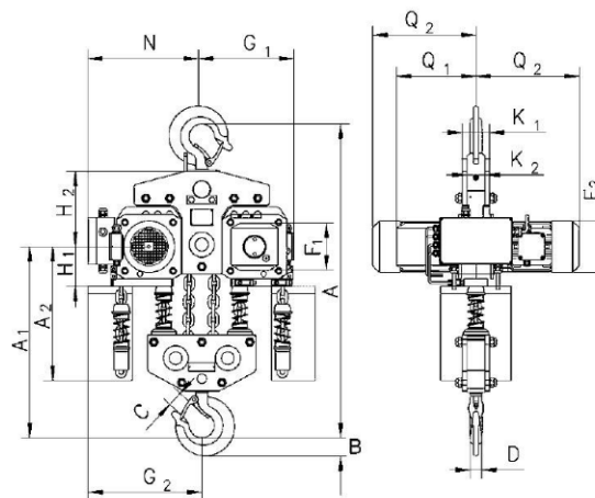
Model CPE/CPEF 100-2 with suspension hook, 10000 kg
