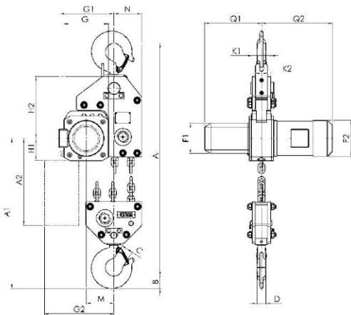
Model CPE/CPEF 75-1,6 with suspension hook, 7500 kg
