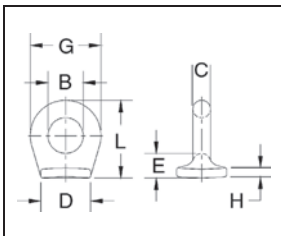
S-264 Pad Eyes
