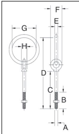
G-257 Shoulder Nut Ring Bolts
